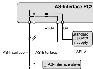
AS-i powered by a standard power supply
