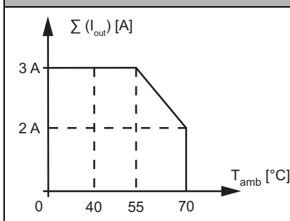
(2) BWU2594, BWU2713, Derating total current of outputs
